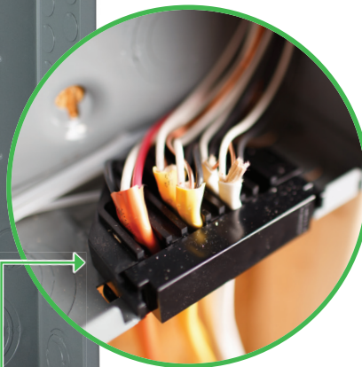
Qwik-Grip Wire Management System
